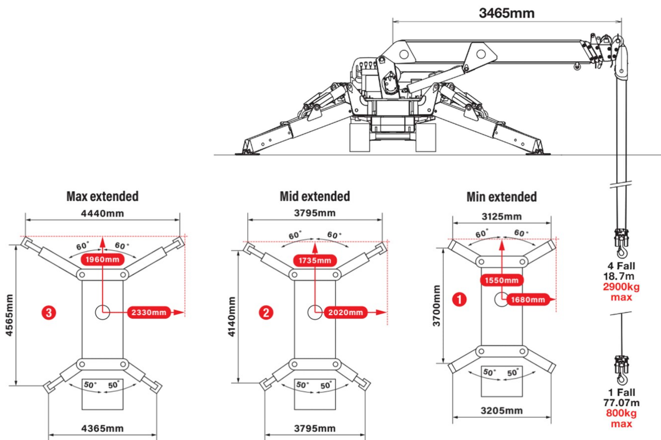
WORKING RANGE & NET RATED LOADS (kg)
