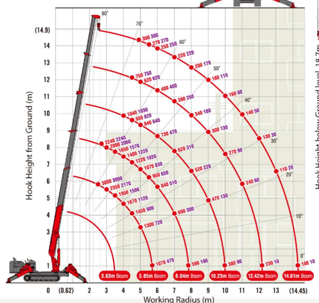
WORKING RANGE & NET RATED LOADS (kg)
